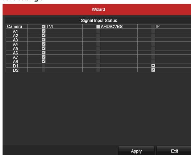
Figure 3.9 Configure Signal Input Type
