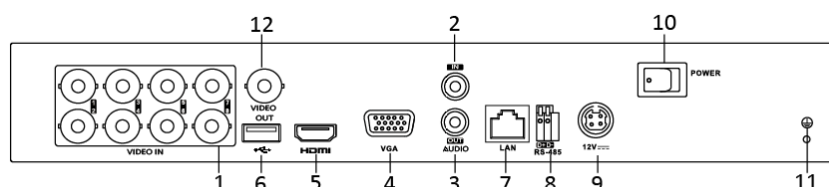
Figure 1.3 Rear Panel
