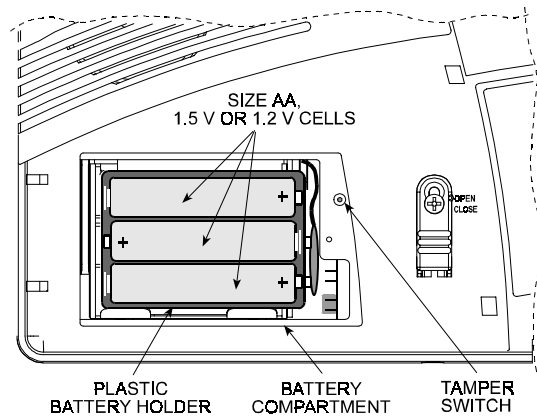
Figure 12. Battery Compartment and Battery Holder
