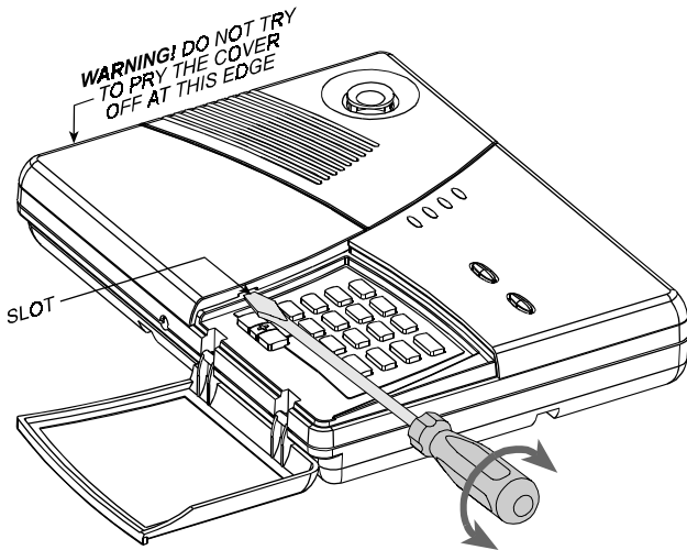
Figure 9. Prying the Cover Loose
