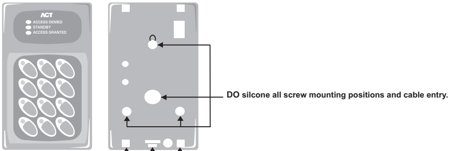
Figure 3: ACT 10 Digital Keypad - Guide to outdoor installation in exposed areas
