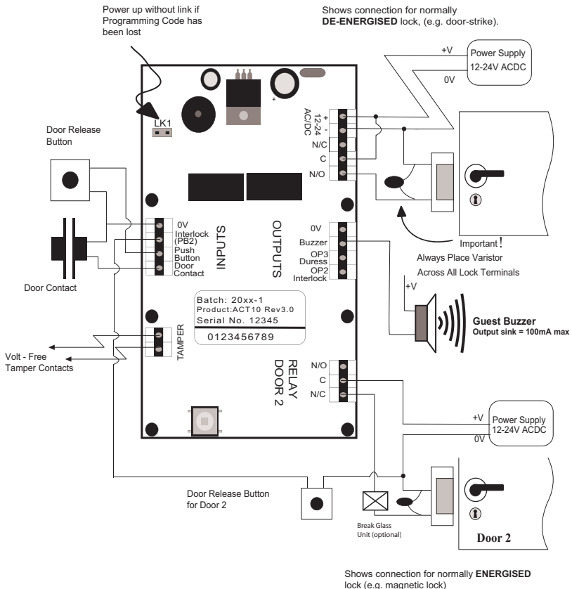
Figure 1: Typical ACT 10 Configuration
